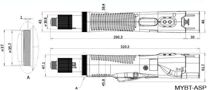
MYBT-ASP Unit: mm
