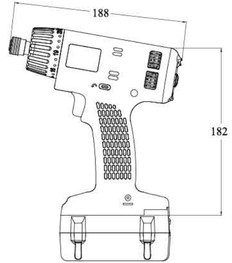
MYBT-SC0612 Unit: mm
